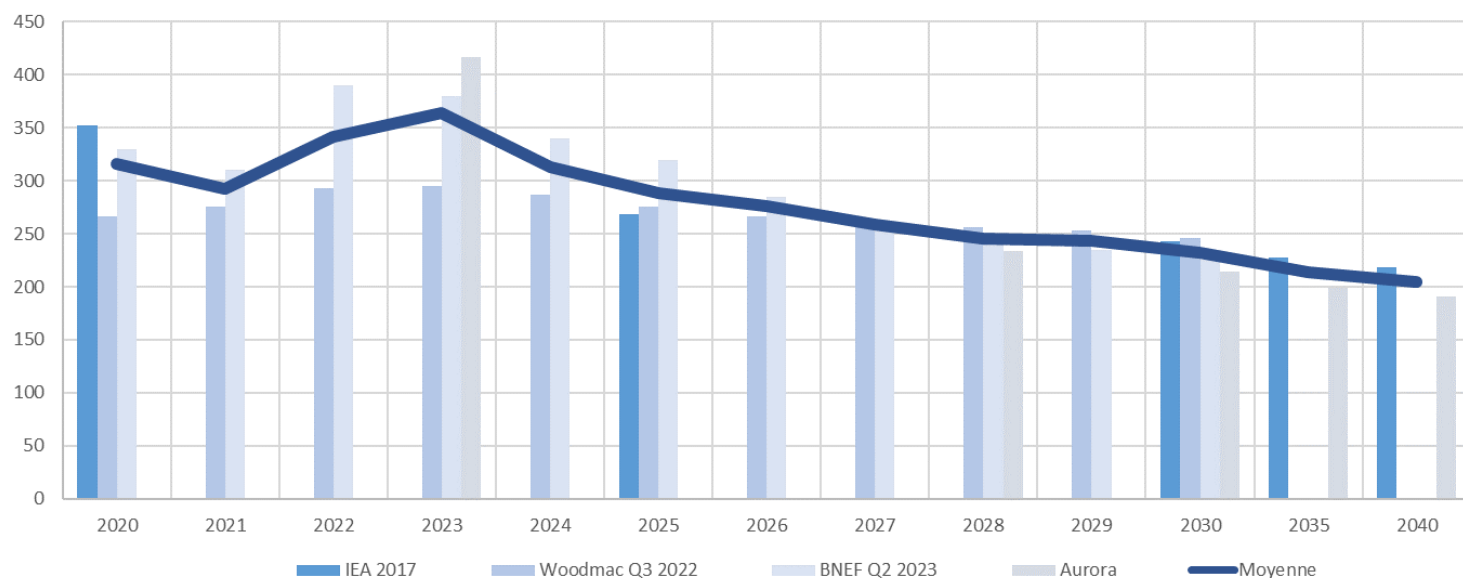
CAPEX Grid-scale Battery 4h - in $/kWh
